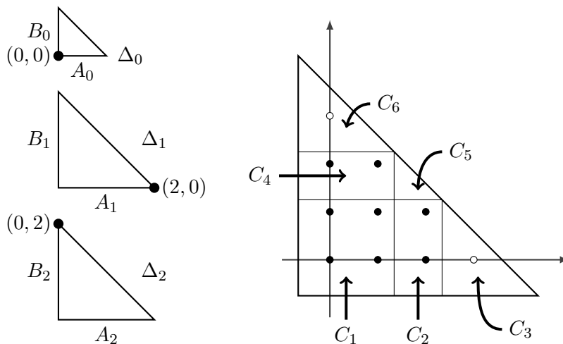
FIGURE 5.4. A non-admissible mixed subdivision
