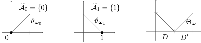
FIGURE 3.2. Convex piecewise affine functions for other subsets
